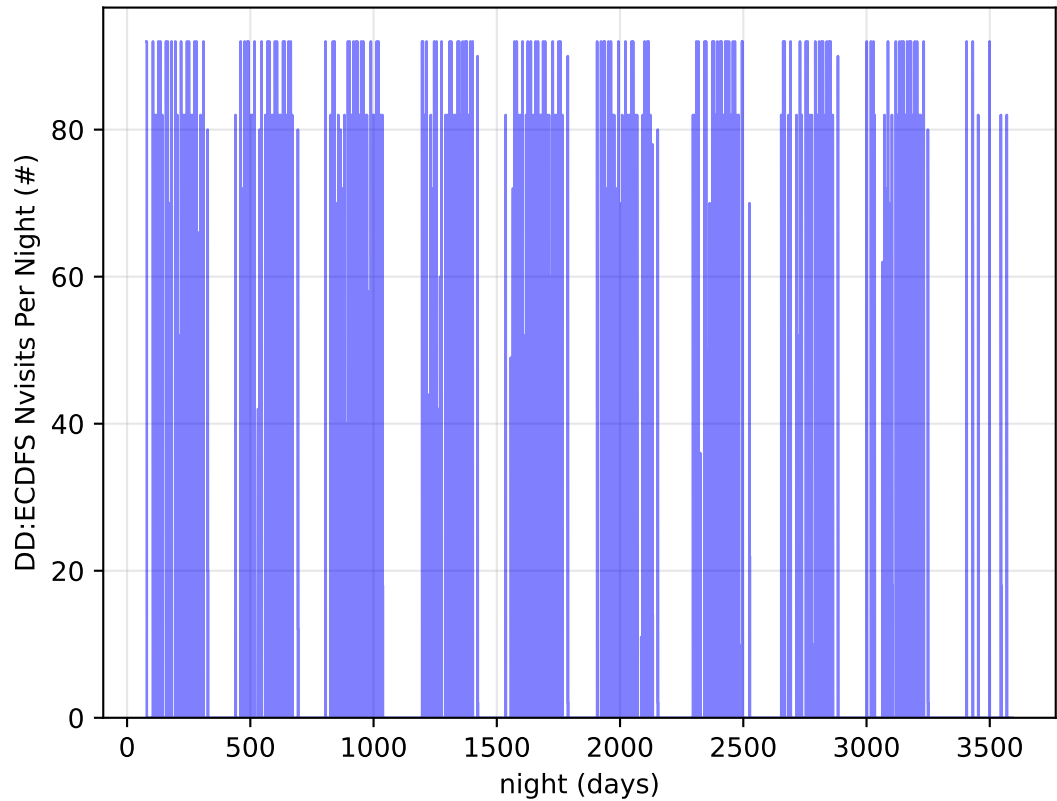
ddf_acor_sf10_ls20_lsr20_v3.4_10yrs all bands: DD:ECDFS Nvisits Per Night
