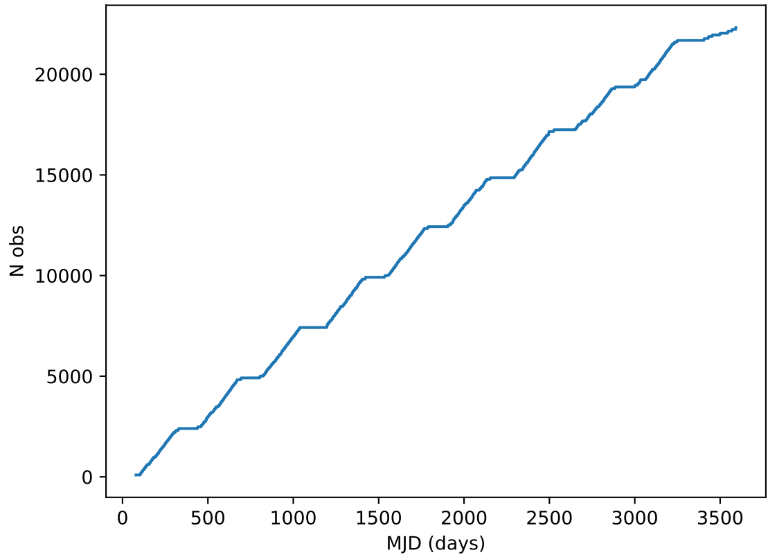
ddf_acor_sf10_lsf20_lsr20_v3.4_10yrs all bands: DD:ECDFS Cumulative NVisits
