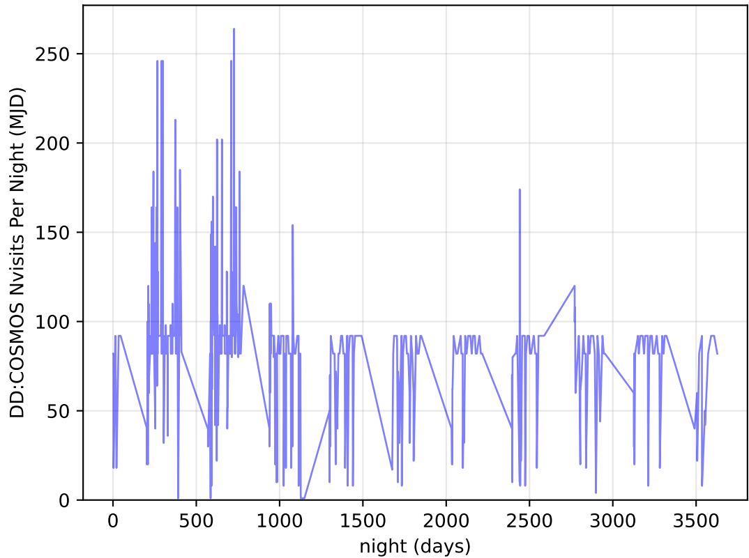
ddf_acor_sf10_lsf20_lsr20_v3.4_10yrs all bands: DD: COSMOS Nvisits Per Night
