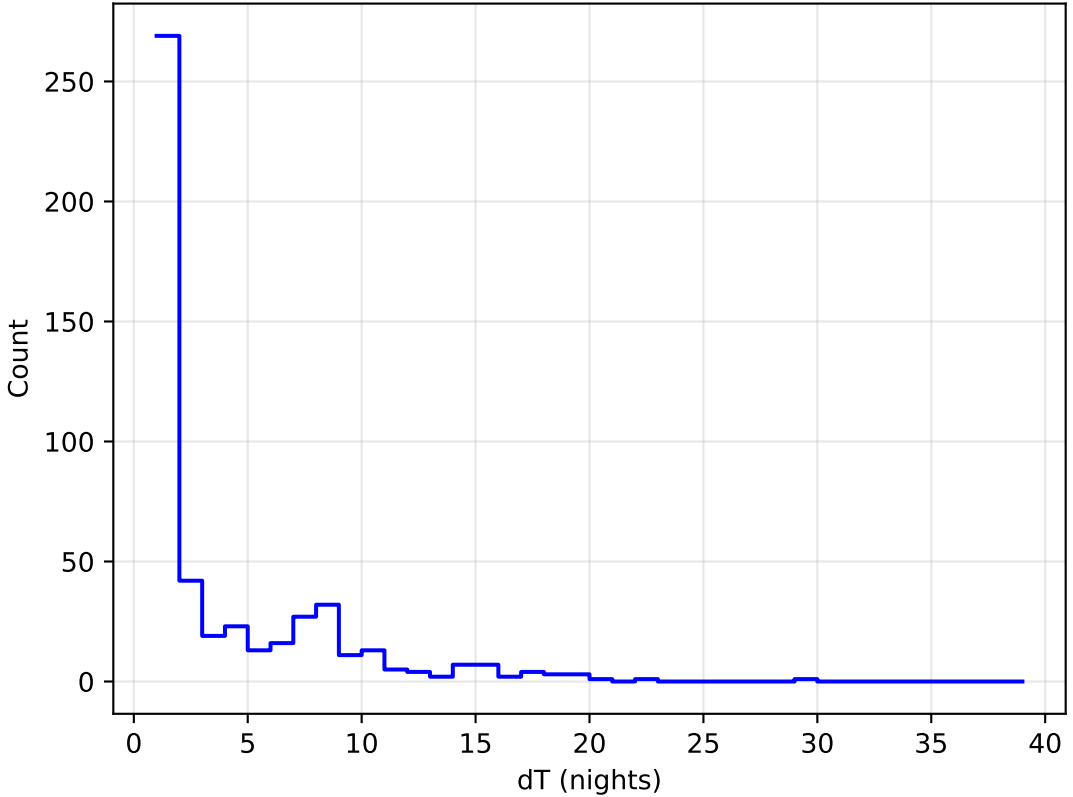
ddf_acor_sf10_lsf20_lsr20_v3.4_10yrs all bands: DD: COSMOS Delta Nights Histogram
