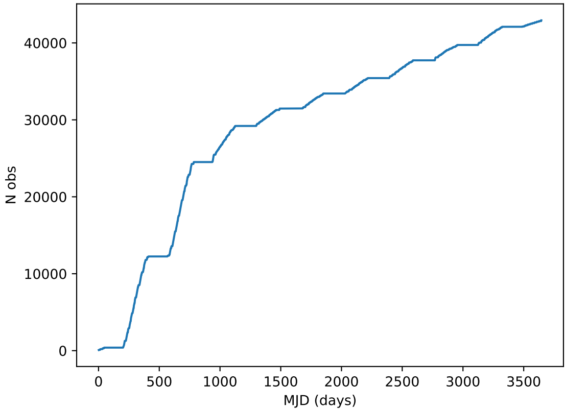
ddf_acor_sf10_lsf20_lsr20_v3.4_10yrs all bands: DD: COSMOS Cumulative NVisits
