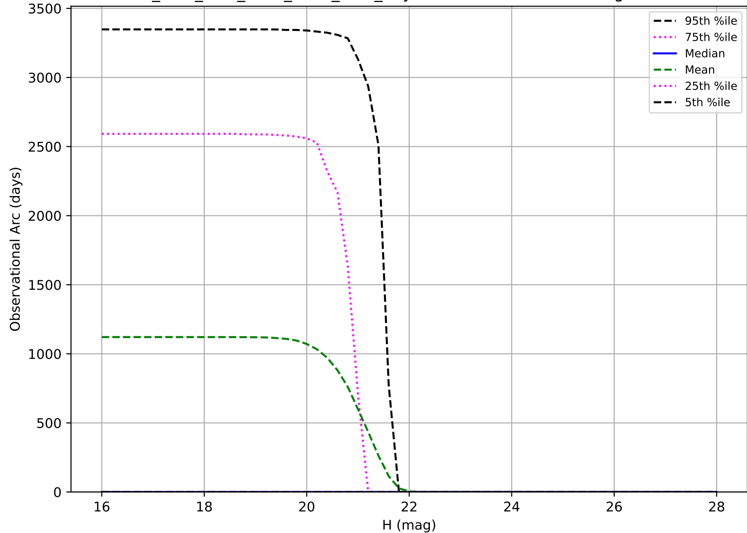
ddf_acor_sf10_lsf20_lsr10_v3.4_10yrs: Observational Arc Length Vatira
