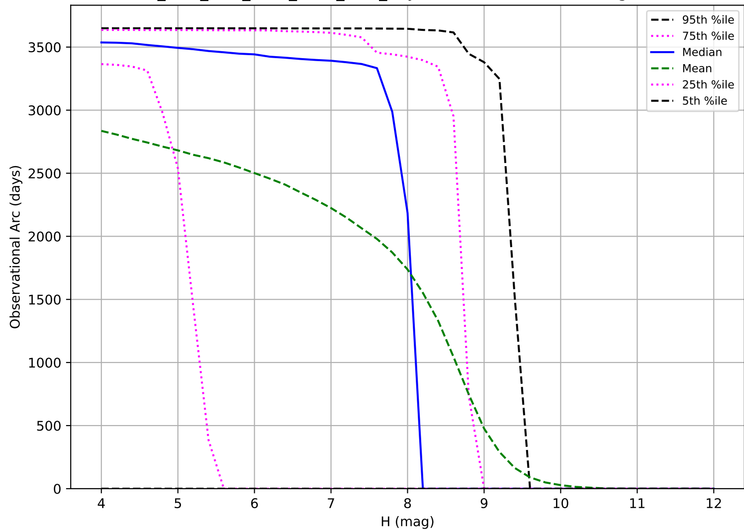
ddf_acor_sf10_lsf20_lsr10_v3.4_10yrs: Observational Arc Length TNO
