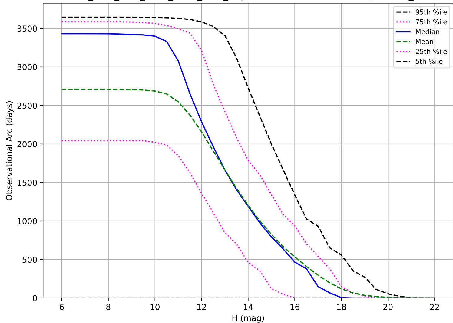
ddf_acor_sf10_lsf20_lsr10_v3.4_10yrs: Observational Arc Length OCC_r5
