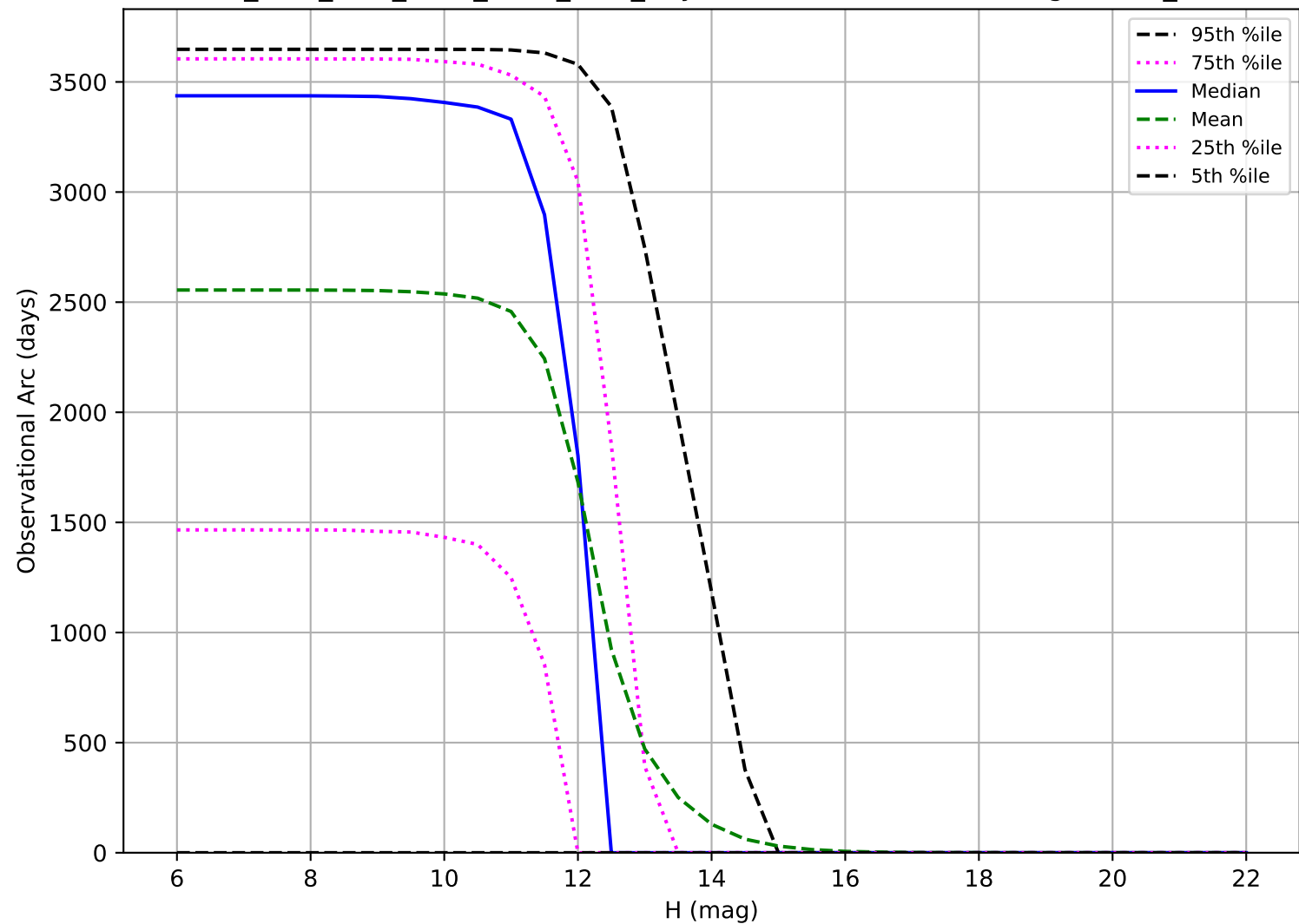
ddf_acor_sf10_lsf20_lsr10_v3.4_10yrs: Observational Arc Length OCC_r20
