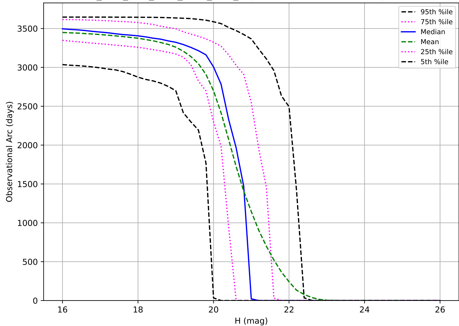
ddf_acor_sf10_lsf20_lsr10_v3.4_10yrs: Observational Arc Length MBA
