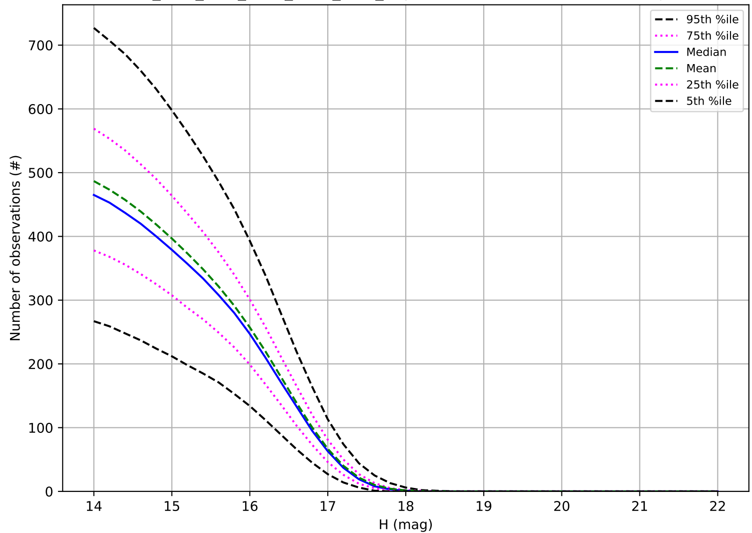
ddf_acor_sf10_lsf20_lsr10_v3.4_10yrs: Number of observations Trojan
