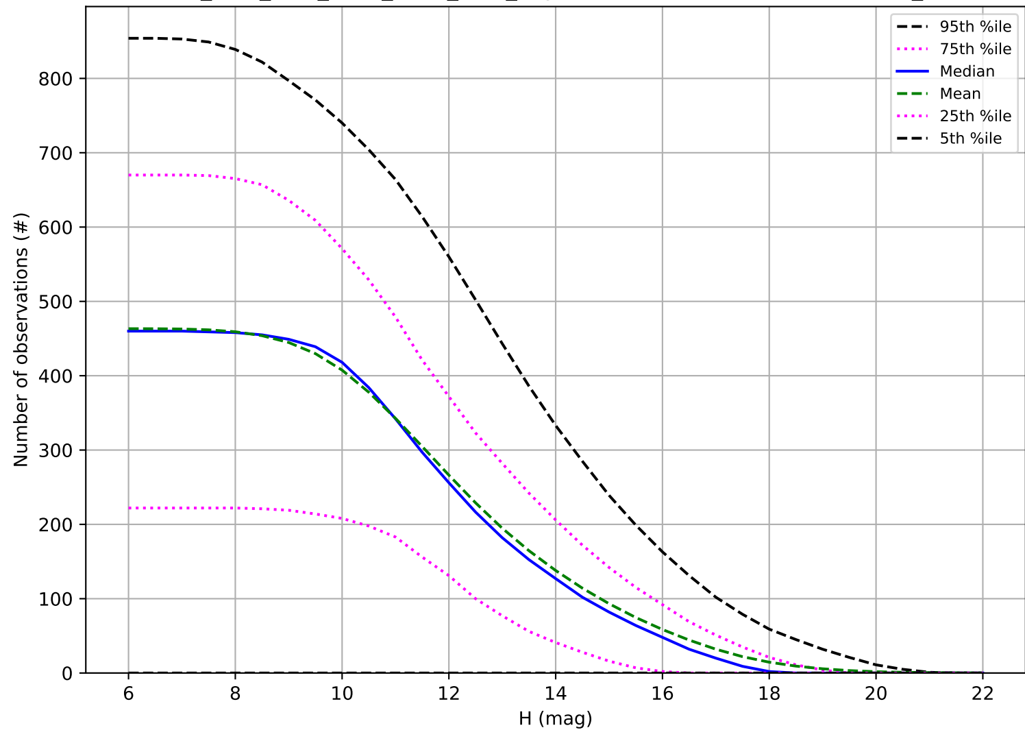
ddf_acor_sf10_lsf20_lsr10_v3.4_10yrs: Number of observations OCC_r5
