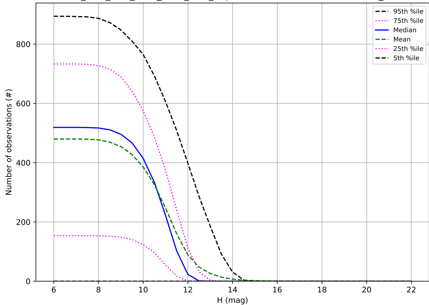
ddf_acor_sf10_lsf20_lsr10_v3.4_10yrs: Number of observations OCC_r20
