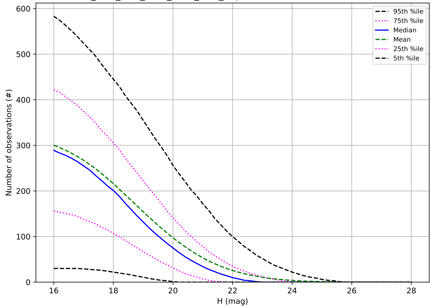
ddf_acor_sf10_lsf20_lsr10_v3.4_10yrs: Number of observations NEO
