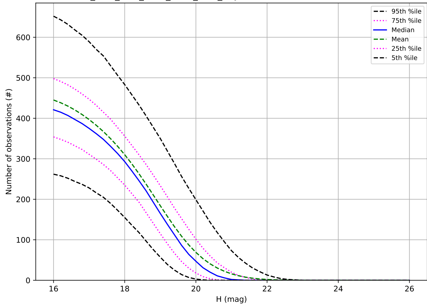
ddf_acor_sf10_lsf20_lsr10_v3.4_10yrs: Number of observations MBA
