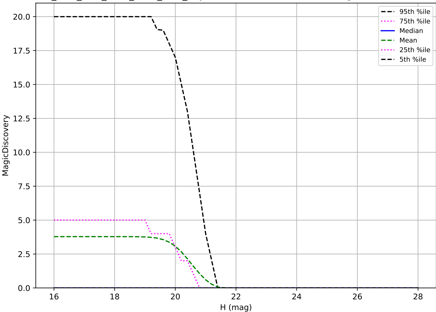
ddf_acor_sf10_lsf20_lsr10_v3.4_10yrs: Vatira 6 detections in 60 nights detection loss
