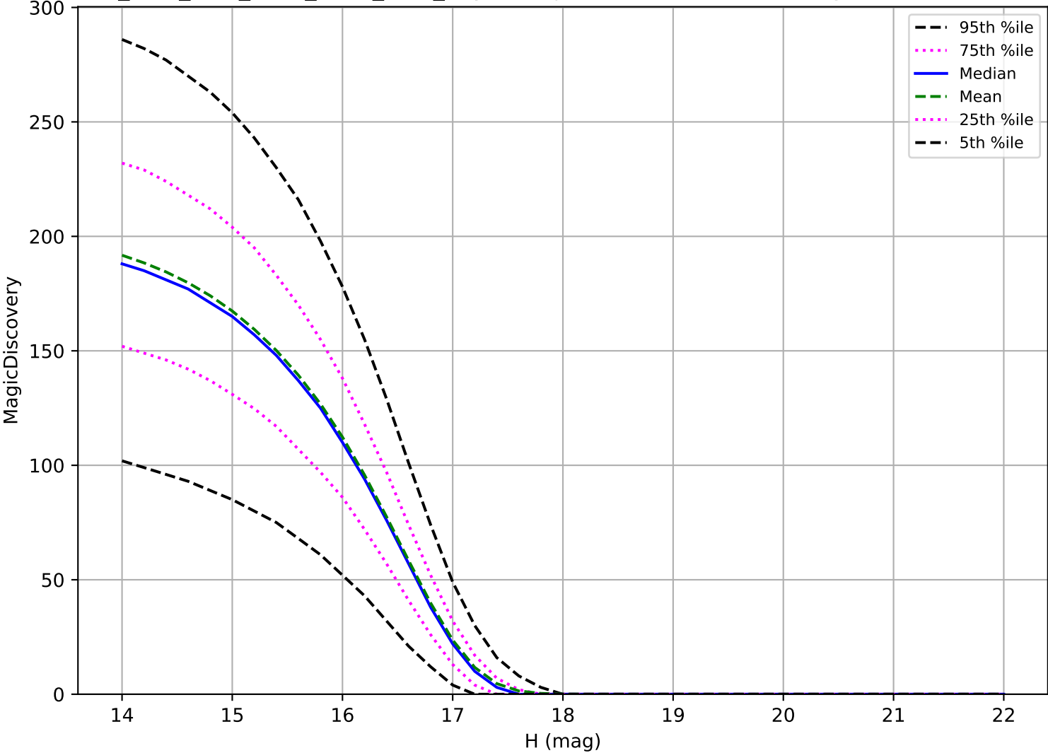
ddf_acor_sf10_lsf20_lsr10_v3.4_10yrs: Trojan 6 detections in 60 nights detection loss
