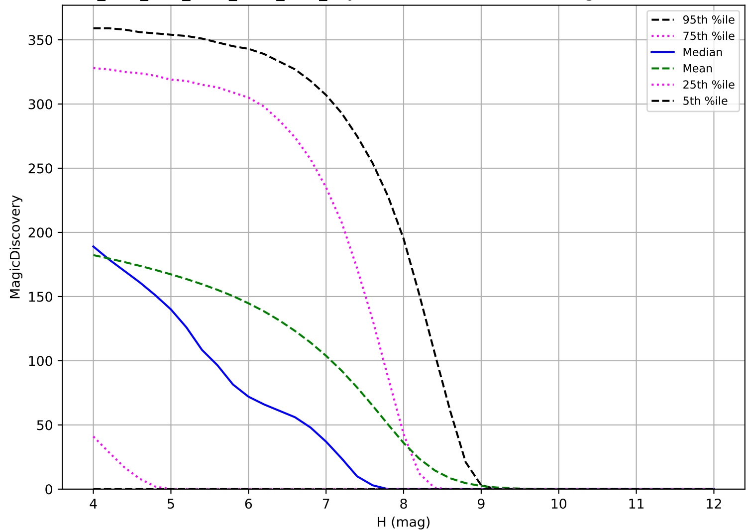
ddf_acor_sf10_lsf20_lsr10_v3.4_10yrs: TNO 6 detections in 60 nights detection loss
