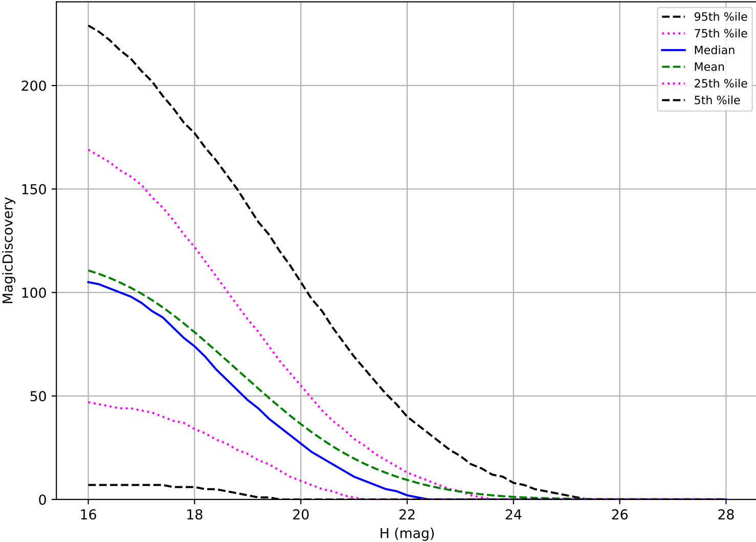
ddf_acor_sf10_lsf20_lsr10_v3.4_10yrs: PHA 6 detections in 60 nights detection loss
