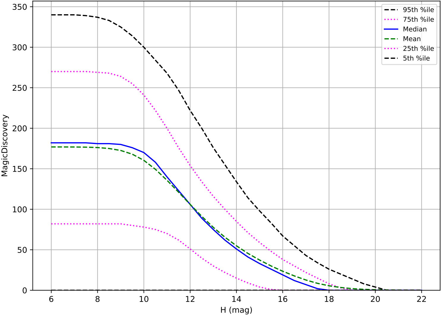
ddf_acor_sf10_lsf20_lsr10_v3.4_10yrs: OCC_r5 6 detections in 60 nights detection loss
