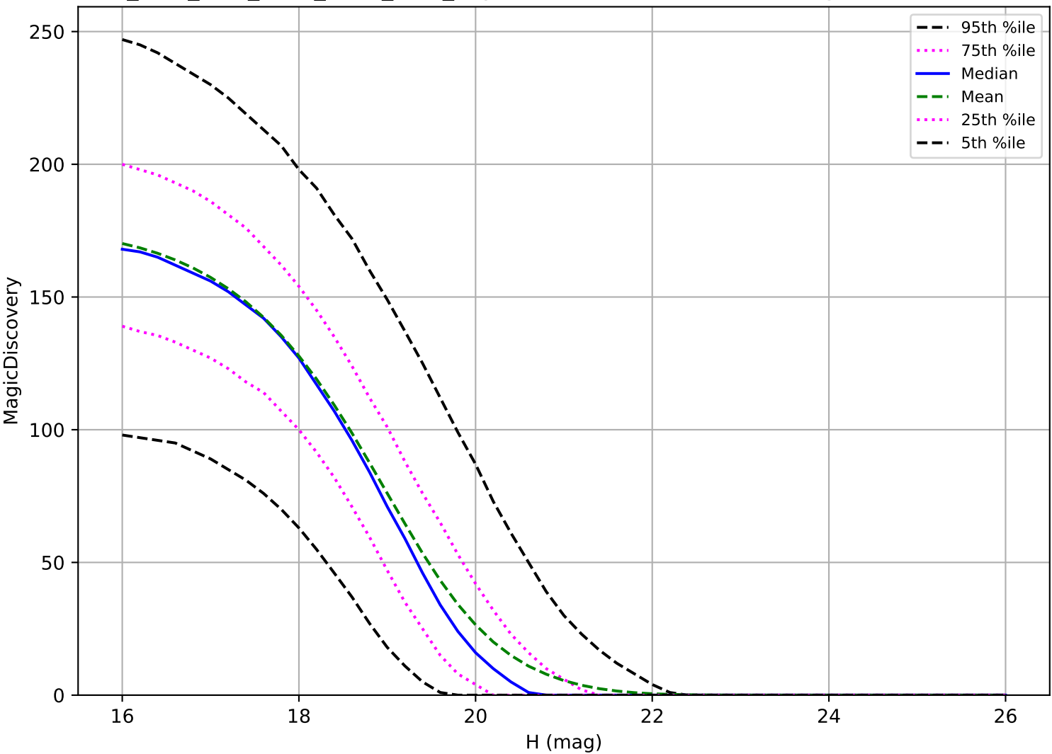
ddf_acor_sf10_lsf20_lsr10_v3.4_10yrs: MBA 6 detections in 60 nights detection loss
