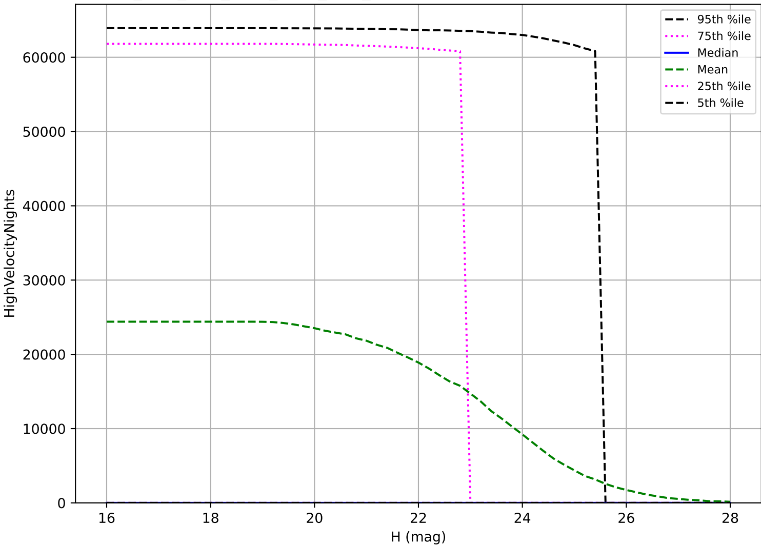
ddf_acor_sf10_lsf20_lsr10_v3.4_10yrs: PHA High velocity pair detection loss
