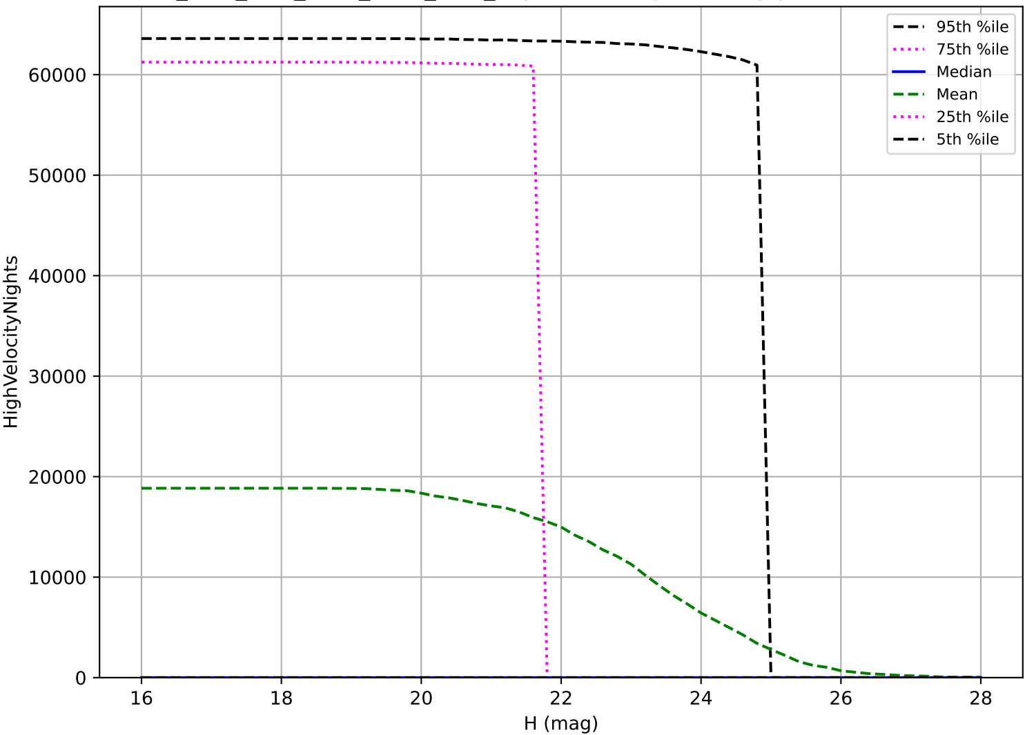
ddf_acor_sf10_lsf20_lsr10_v3.4_10yrs: NEO High velocity pair detection loss
