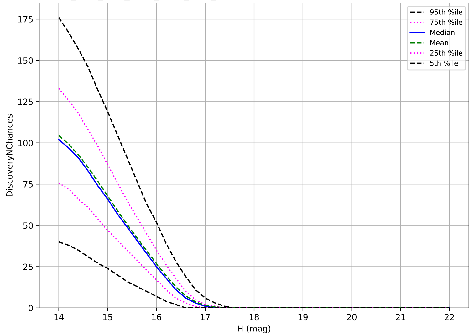
ddf_acor_sf10_lsf20_lsr10_v3.4_10yrs: Trojan 3 pairs in 15 nights detection loss
