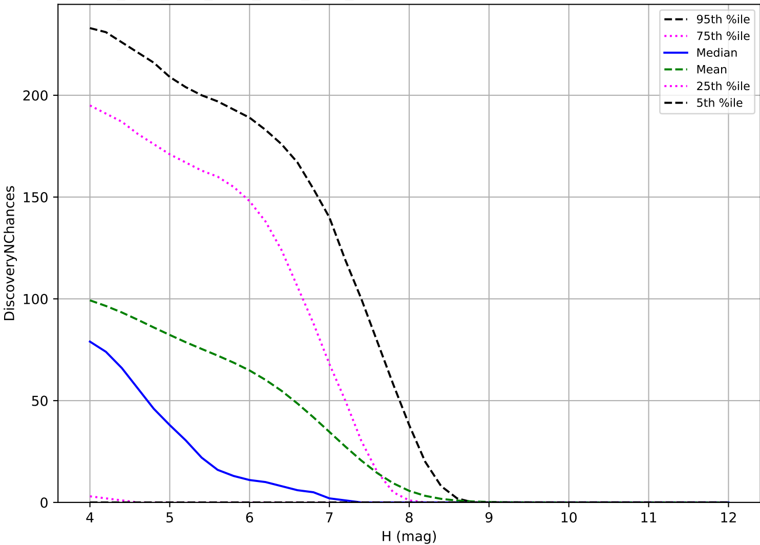
ddf_acor_sf10_lsf20_lsr10_v3.4_10yrs: TNO 3 pairs in 15 nights detection loss
