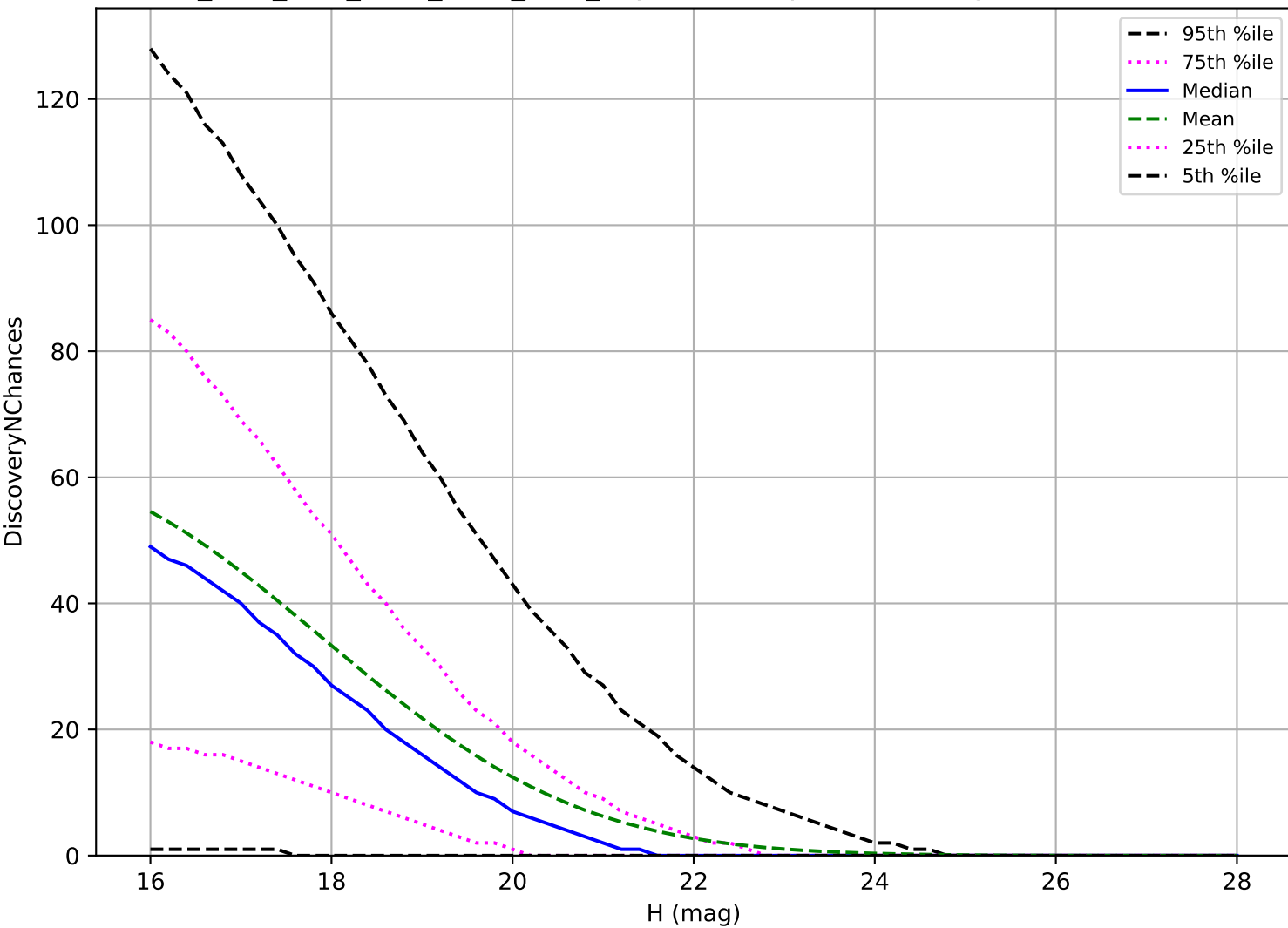
ddf_acor_sf10_lsf20_lsr10_v3.4_10yrs: PHA 3 pairs in 15 nights detection loss
