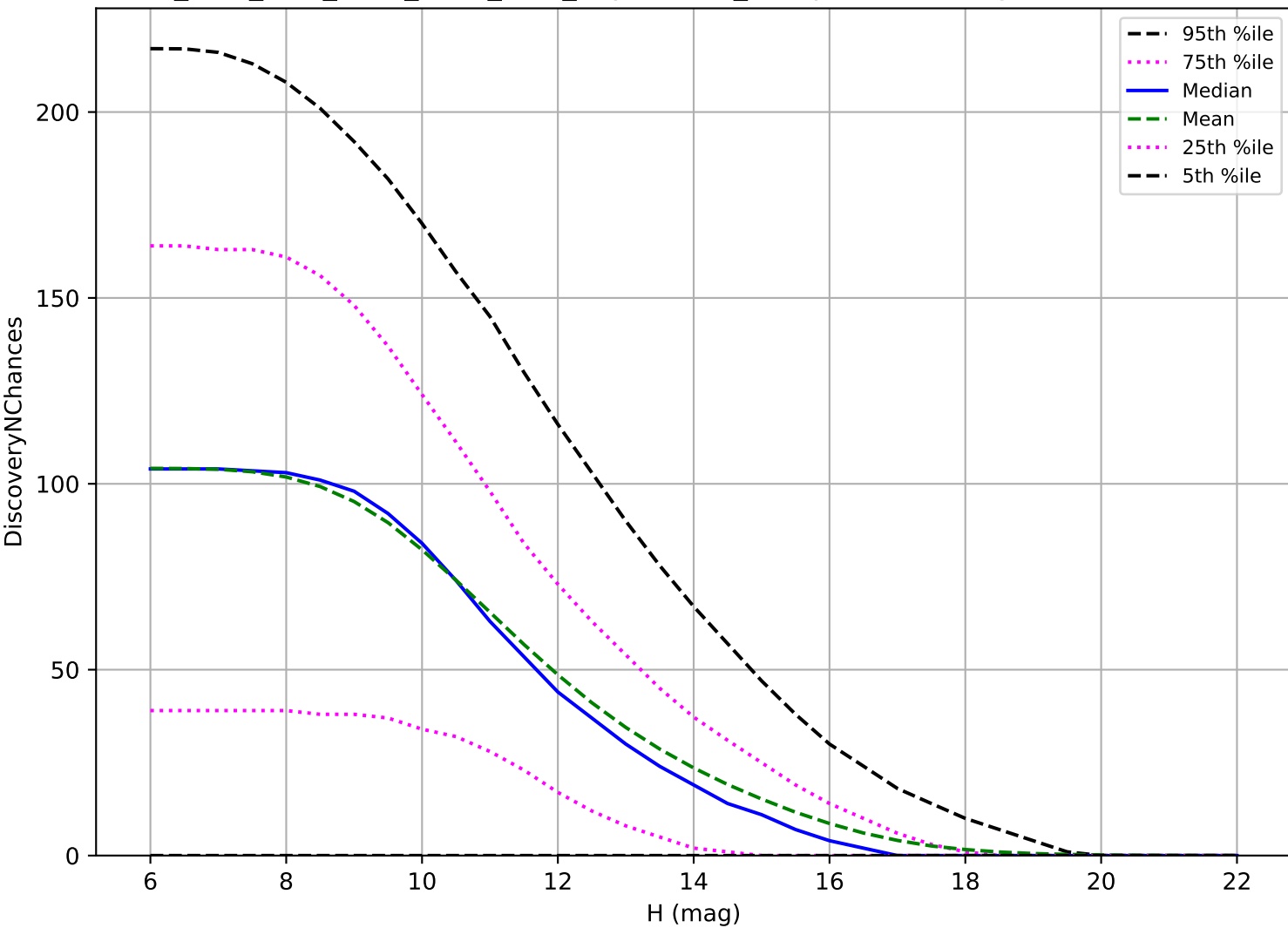
ddf_acor_sf10_lsf20_lsr10_v3.4_10yrs: OCC_r5 3 pairs in 15 nights detection loss
