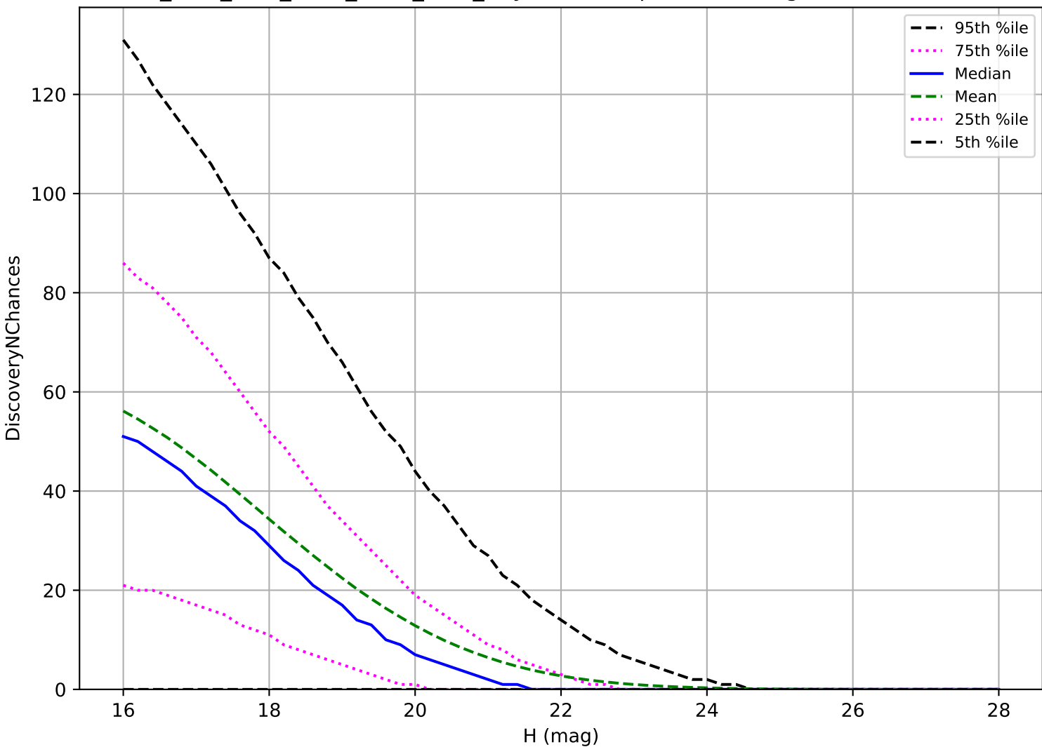
ddf_acor_sf10_lsf20_lsr10_v3.4_10yrs: NEO 3 pairs in 15 nights detection loss
