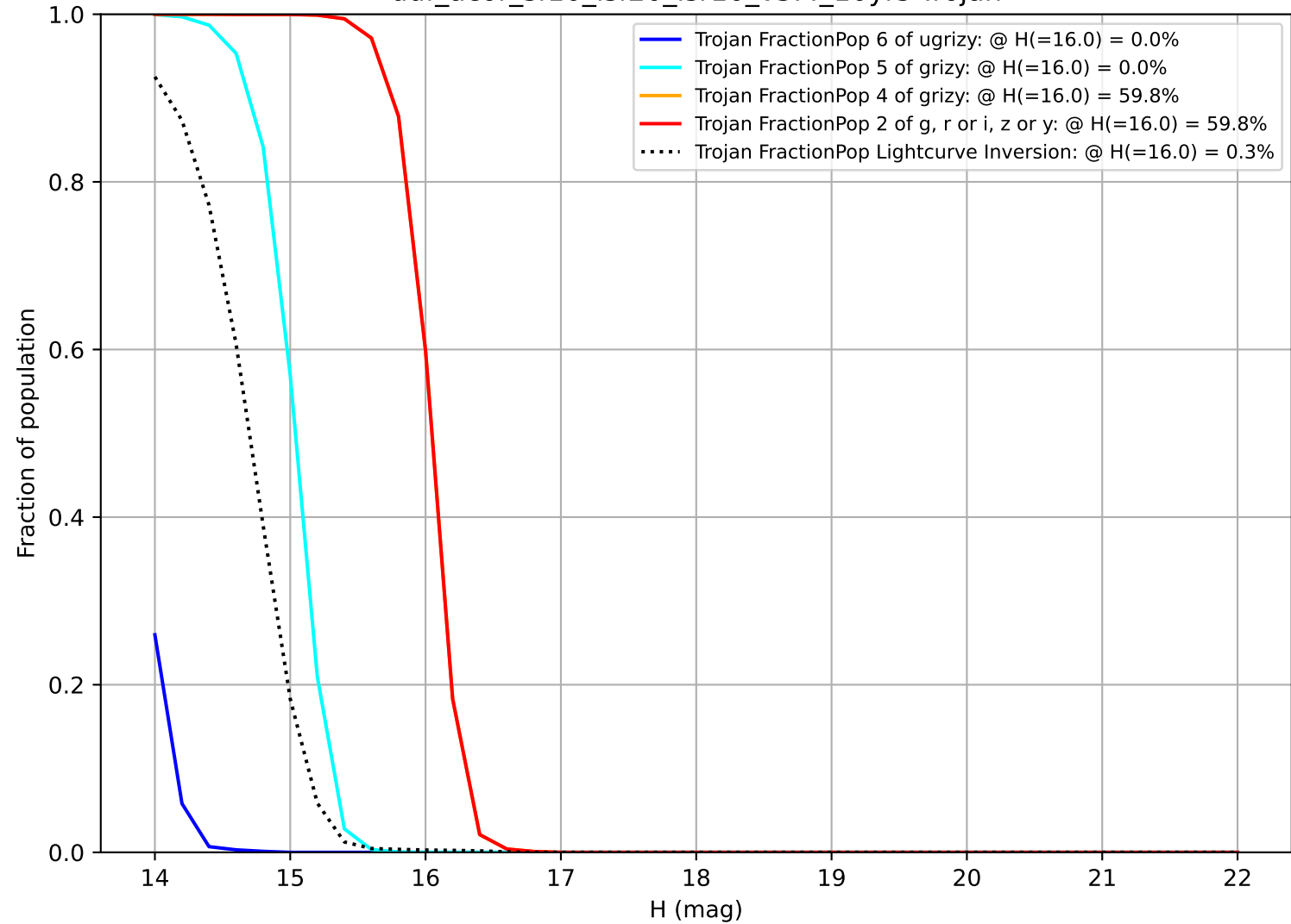
ddf_acor_sf10_lsf20_lsr10_v3.4_10yrs Trojan
