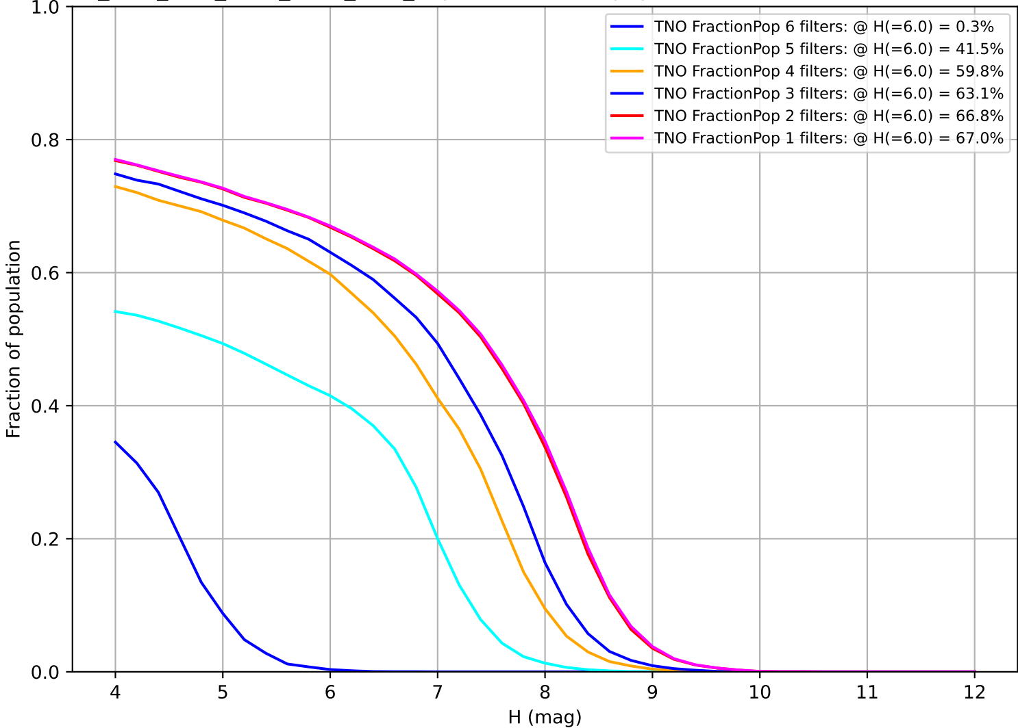
ddf_acor_sf10_lsf20_lsr10_v3.4_10yrs: Fraction of population with colors in X filters TNO
