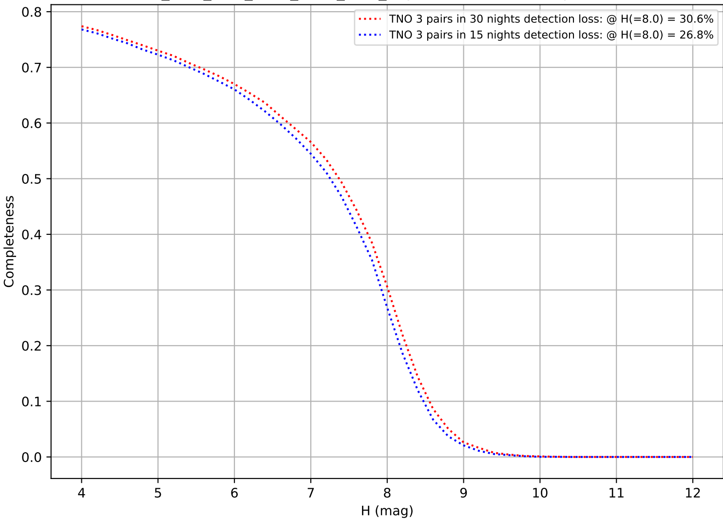
ddf_acor_sf10_lsf20_lsr10_v3.4_10yrs: DifferentialCompleteness
