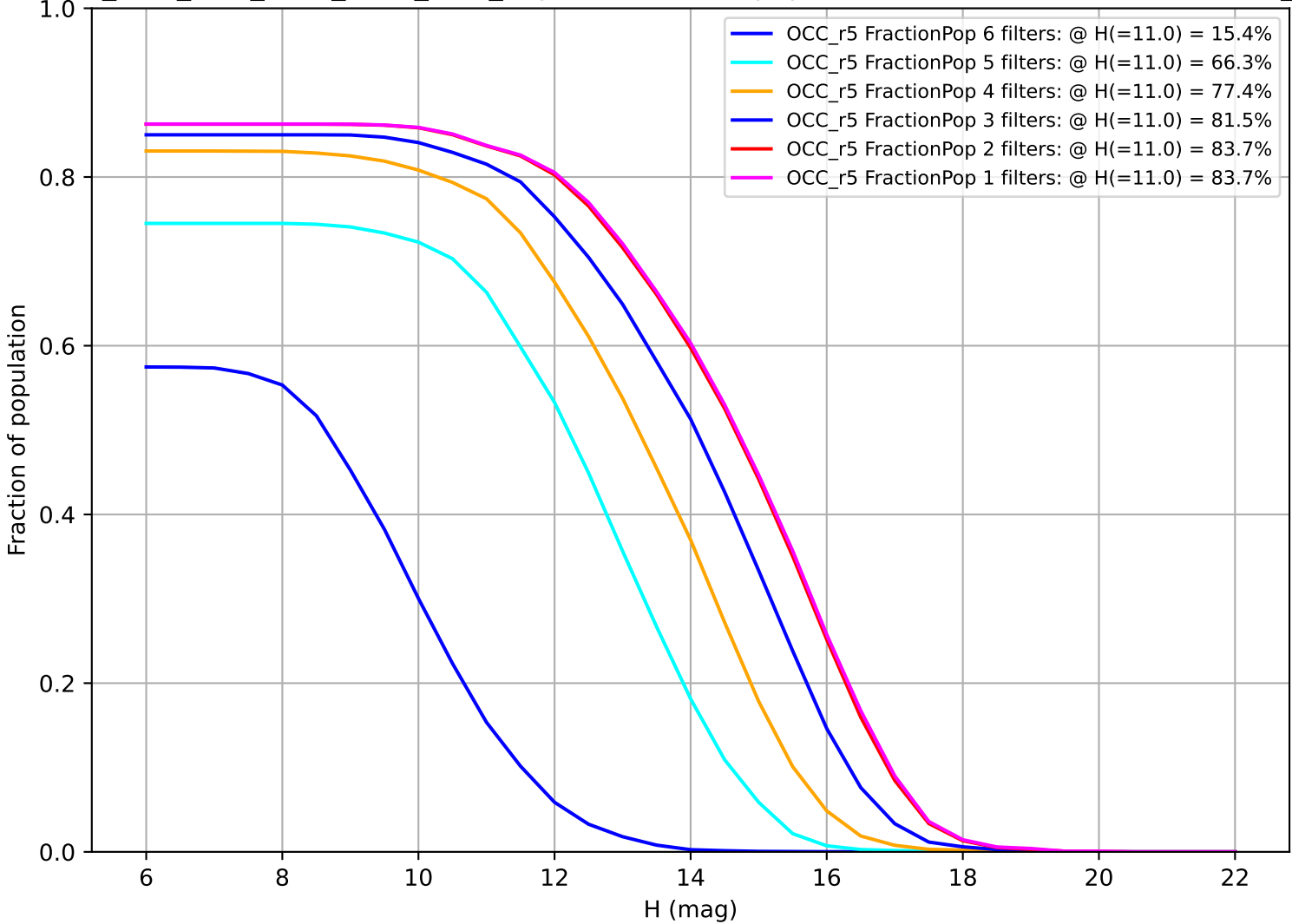
ddf_acor_sf10_lsf20_lsr10_v3.4_10yrs: Fraction of population with colors in X filters OCC_r5
