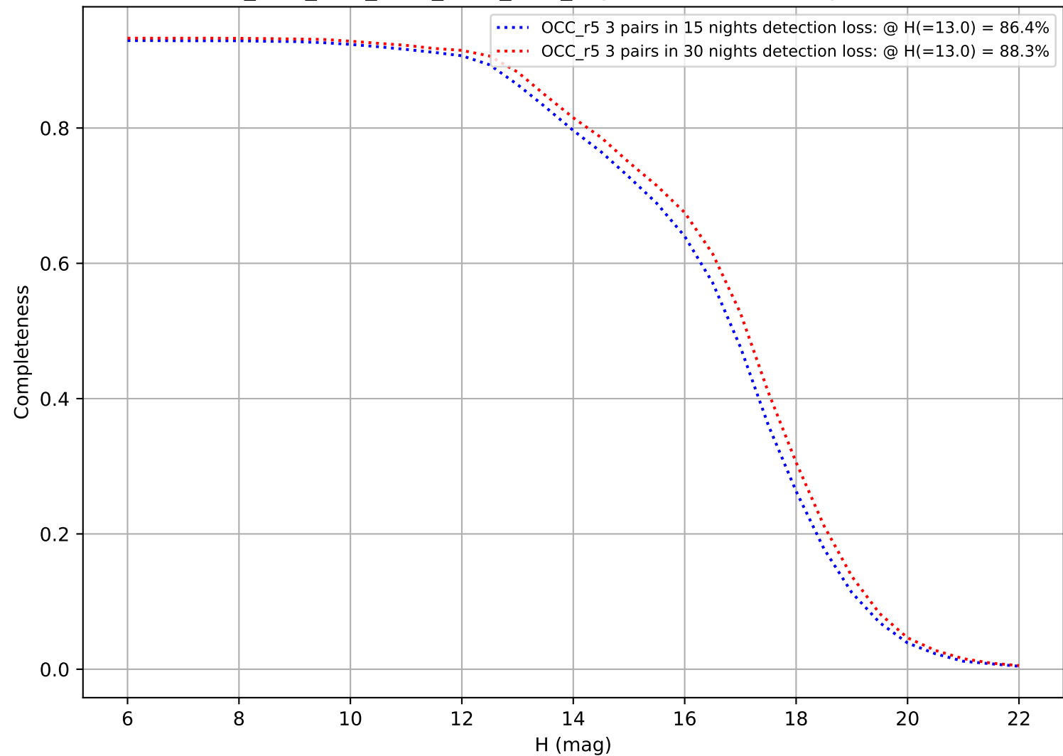
ddf_acor_sf10_lsf20_lsr10_v3.4_10yrs: DifferentialCompleteness
