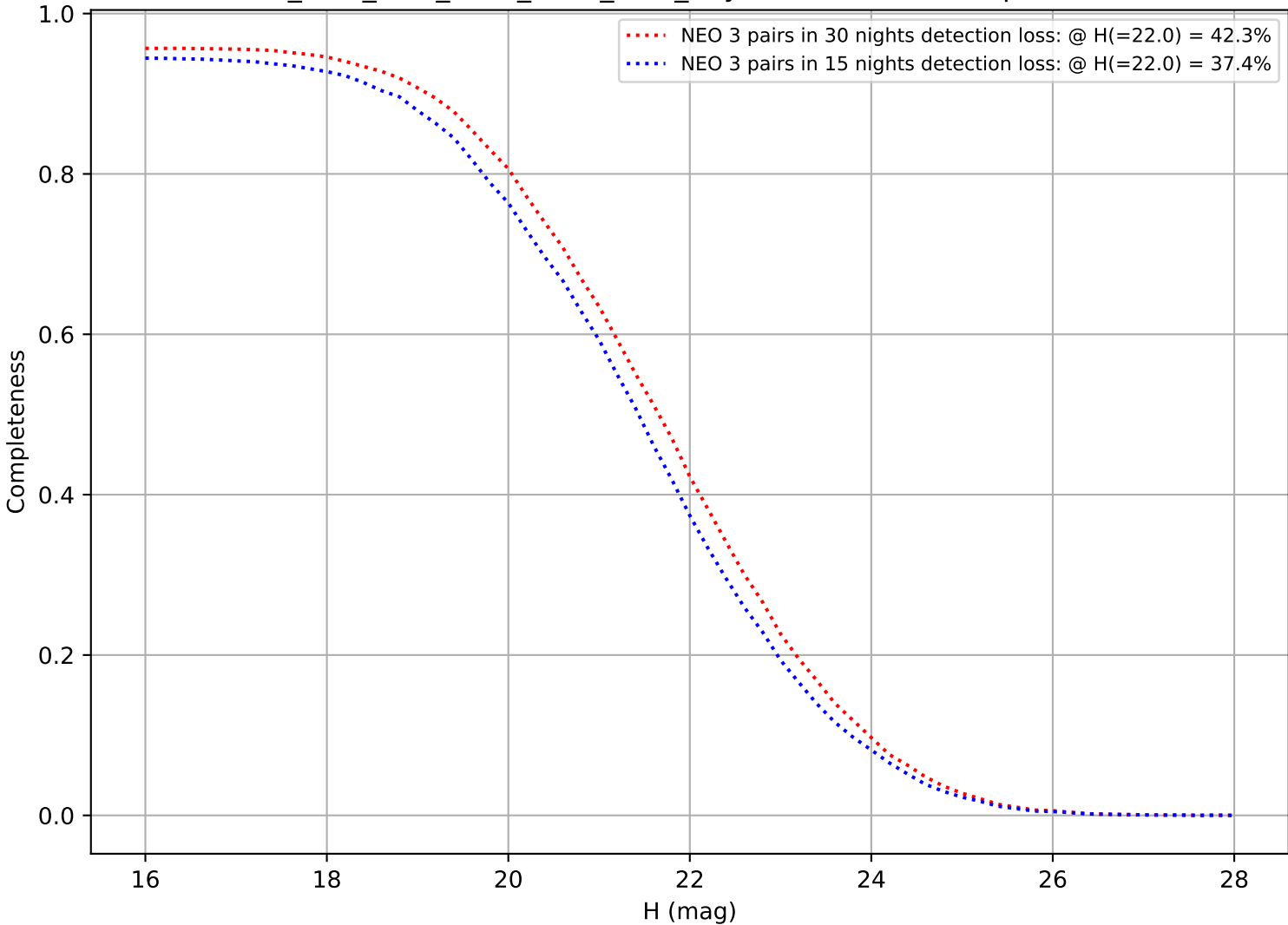
ddf_acor_sf10_lsf20_lsr10_v3.4_10yrs: DifferentialCompleteness
