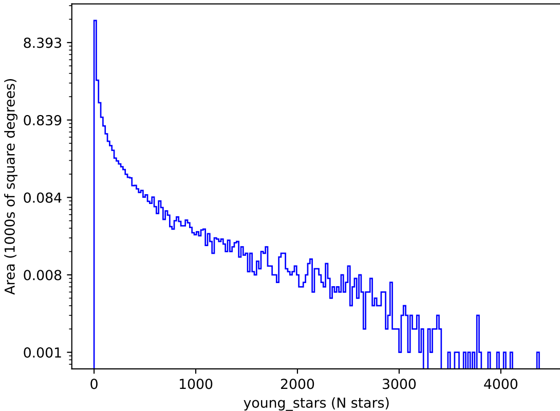
ddf_acor_sf10_lsf20_lsr10_v3.4_10yrs : young_stars
