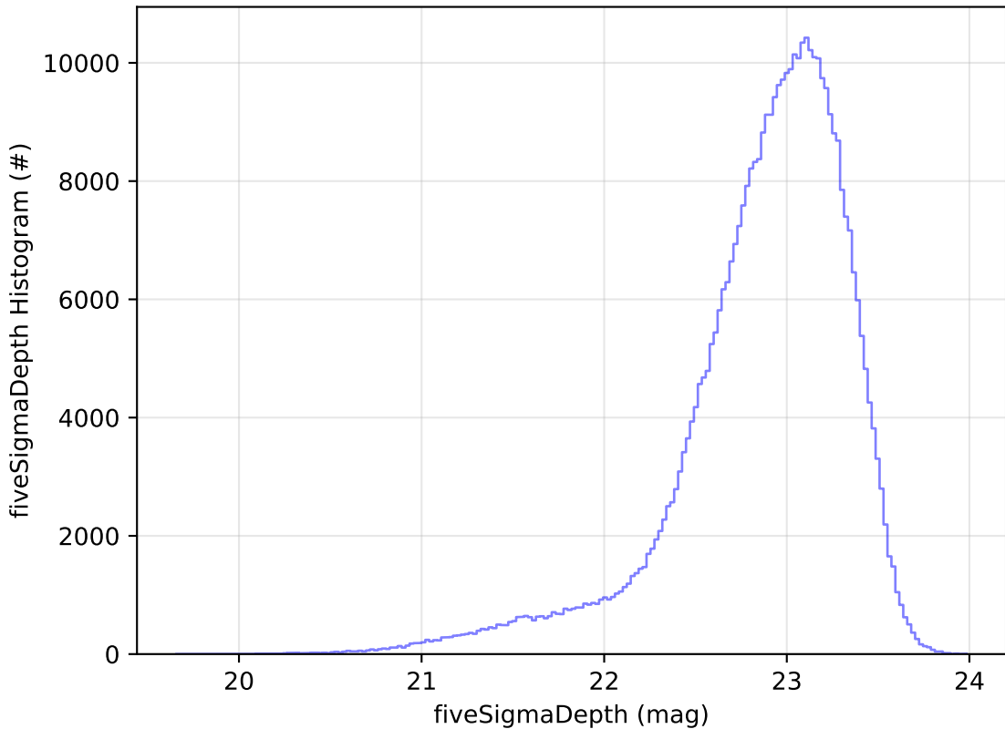
ddf_acor_sf10_lsf20_lsr10_v3.4_10yrs z: fiveSigmaDepth Histogram
