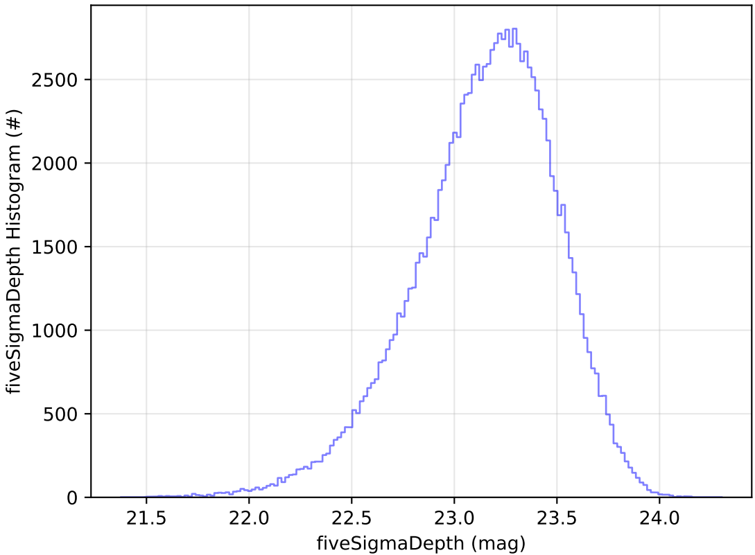
ddf_acor_sf10_lsf20_lsr10_v3.4_10yrs u: fiveSigmaDepth Histogram
