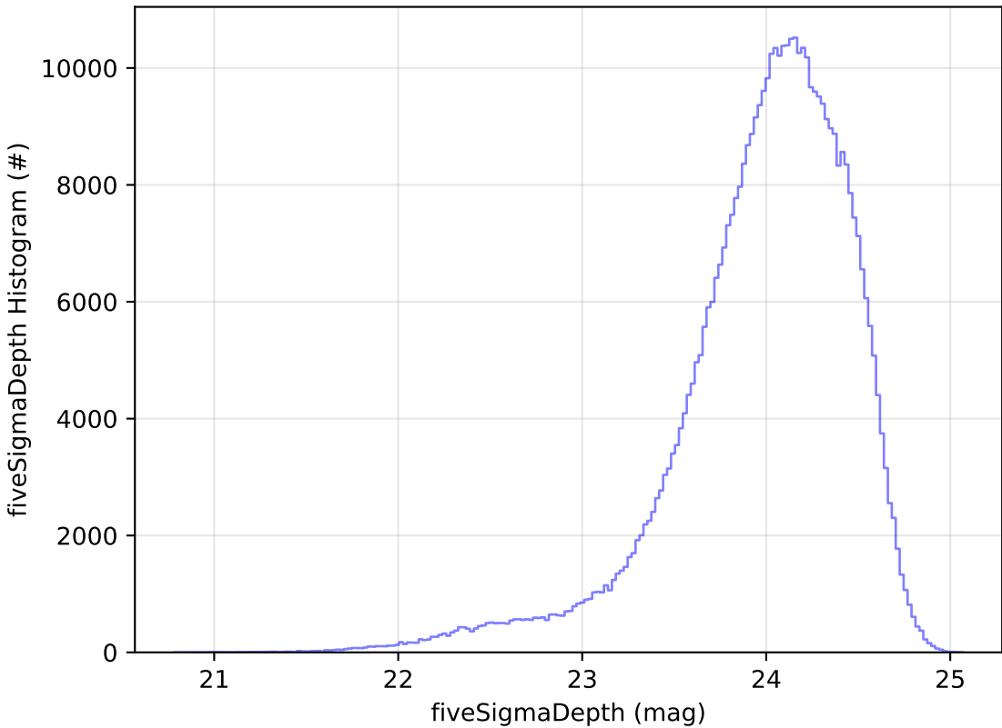
ddf_acor_sf10_lsf20_lsr10_v3.4_10yrs r: fiveSigmaDepth Histogram
