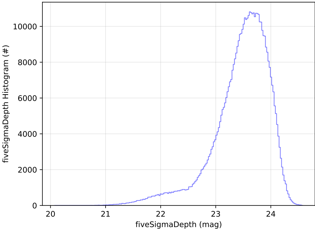
ddf_acor_sf10_lsf20_lsr10_v3.4_10yrs i: fiveSigmaDepth Histogram
