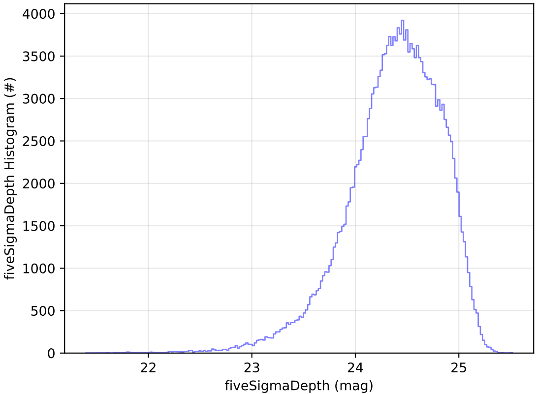
ddf_acor_sf10_lsf20_lsr10_v3.4_10yrs g: fiveSigmaDepth Histogram
