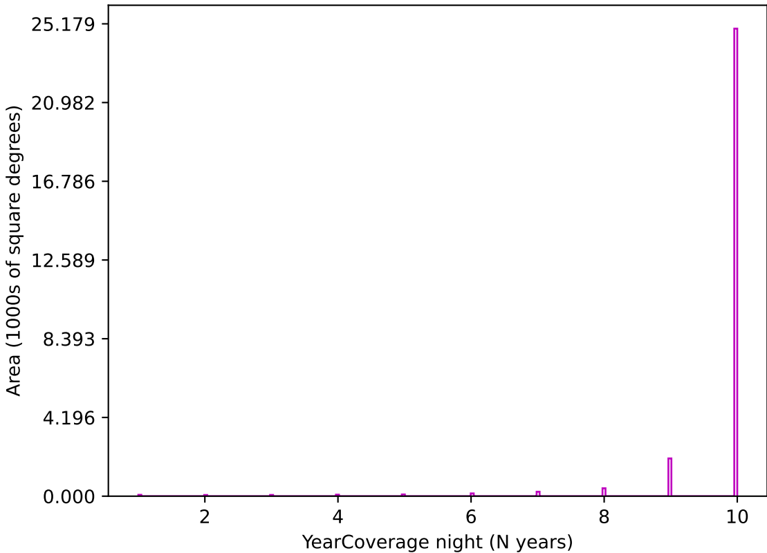
ddf_acor_sf10_lsf20_lsr10_v3.4_10yrs z band: YearCoverage night
