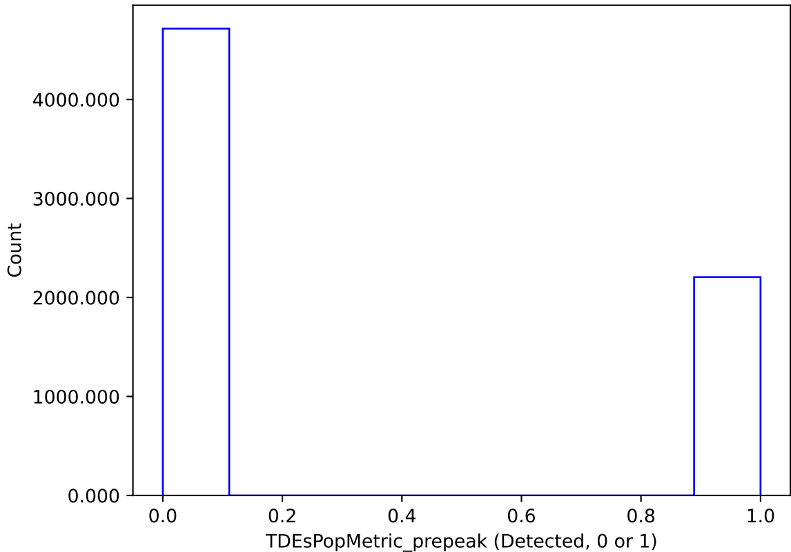
ddf_acor_sf10_lsf20_lsr10_v3.4_10yrs : TDEsPopMetric_prepeak
