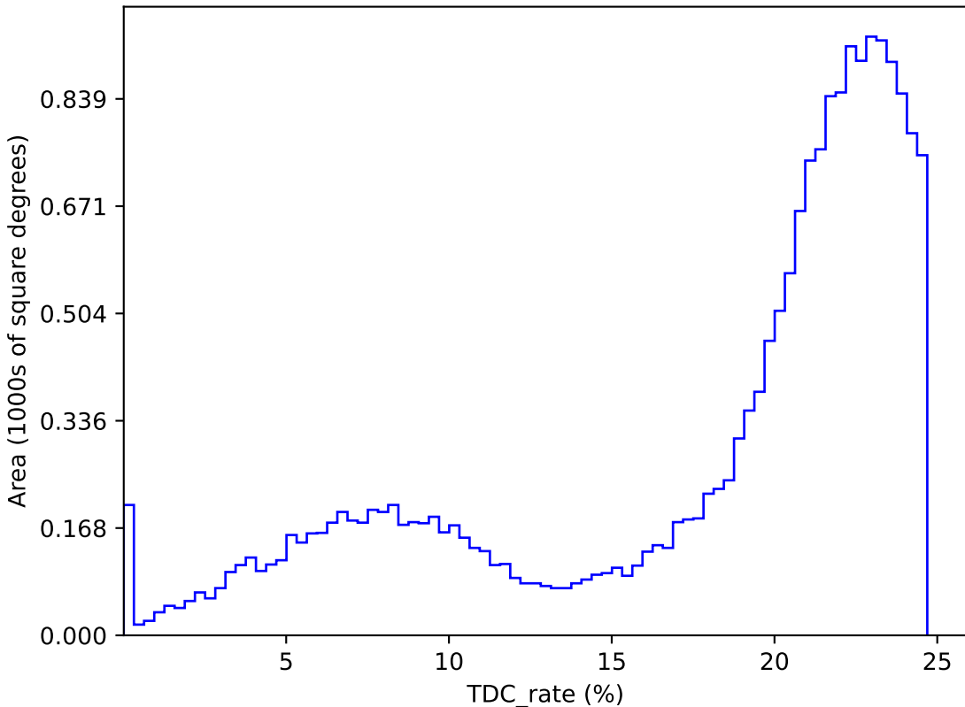
ddf_acor_sf10_lsf20_lsr10_v3.4_10yrs : TDC_rate
