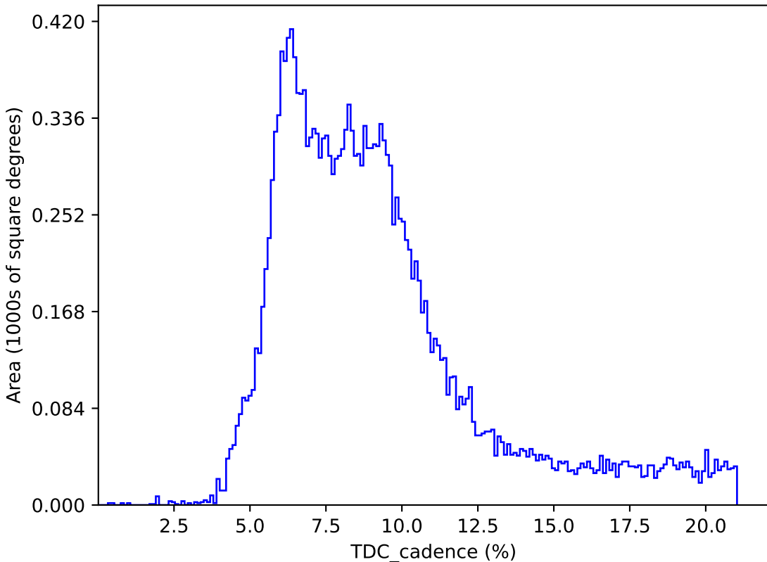
ddf_acor_sf10_lsf20_lsr10_v3.4_10yrs : TDC_cadence
