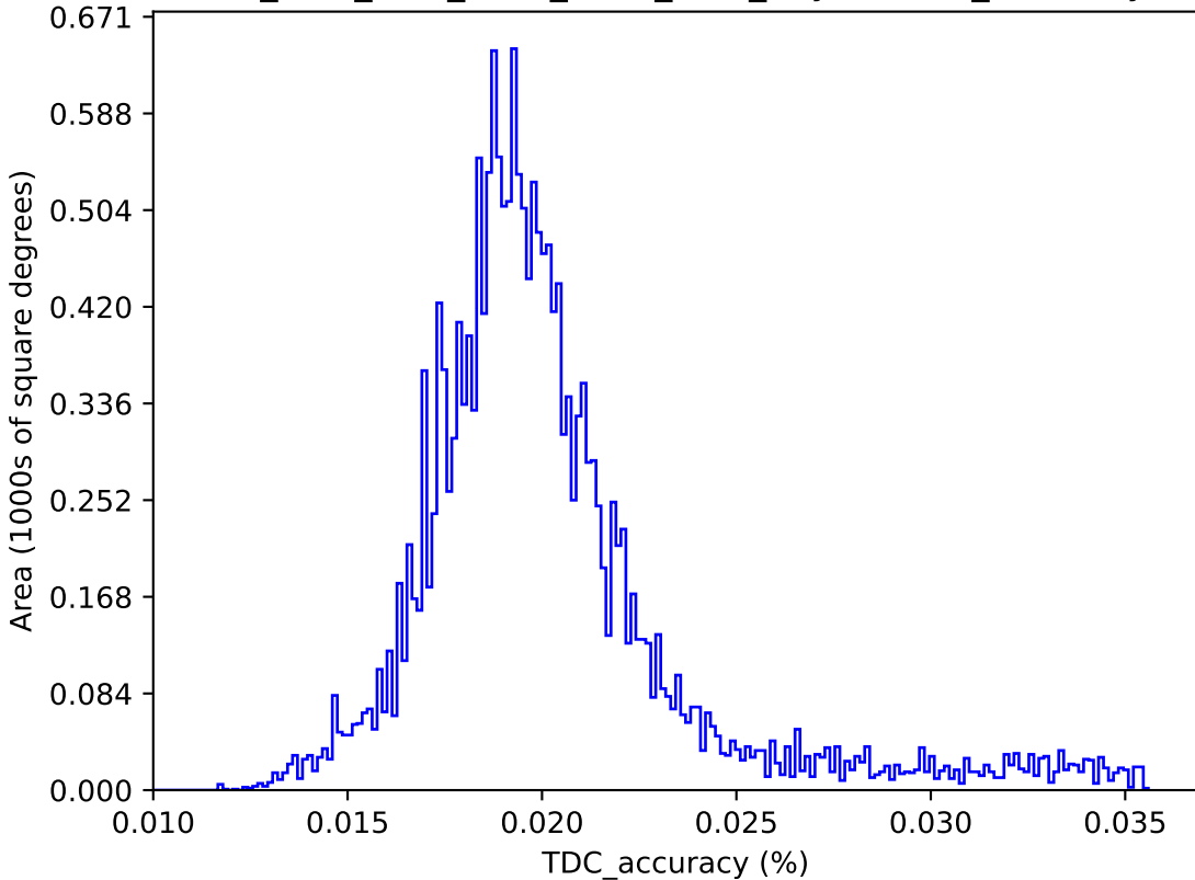
ddf_acor_sf10_lsf20_lsr10_v3.4_10yrs : TDC_accuracy
