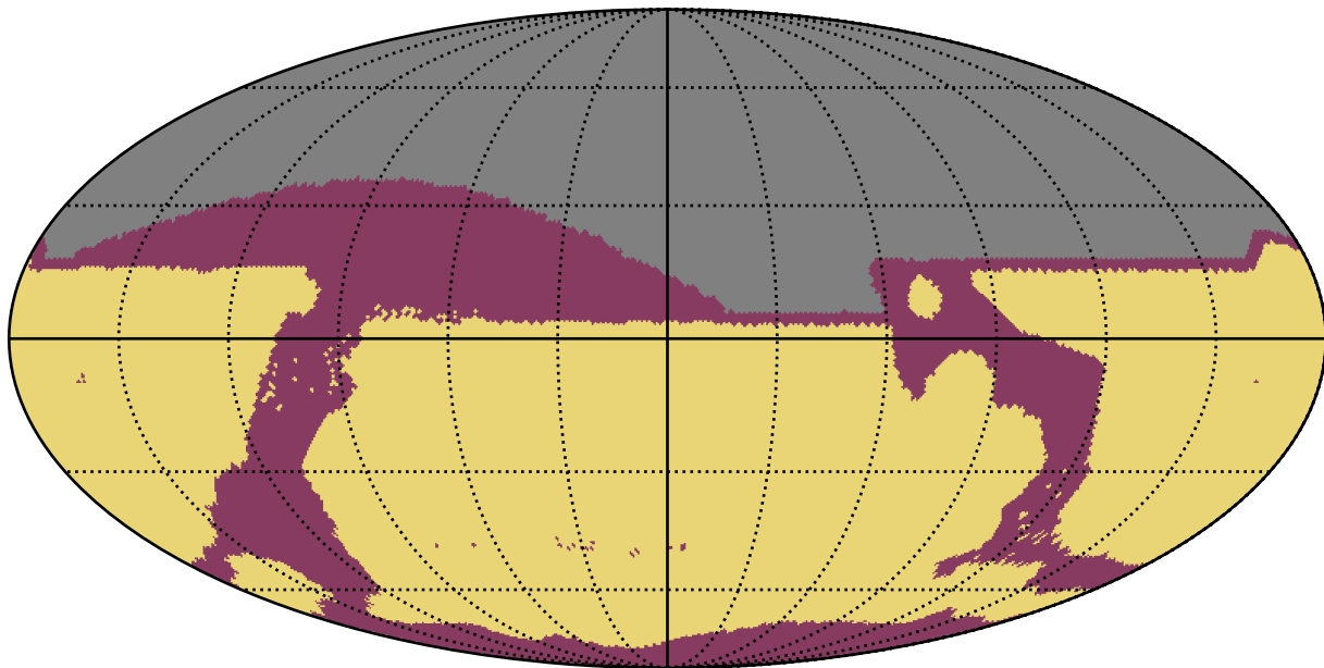
ddf_acor_sf10_lsf20_lsr10_v3.4_10yrs : RapidRevisits
