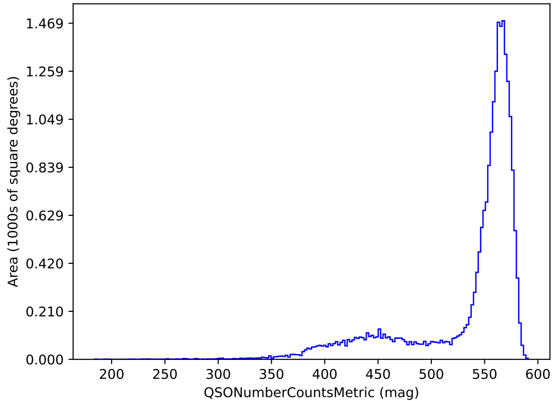
ddf_acor_sf10_lsf20_lsr10_v3.4_10yrs y band and non-DD: QSONumberCountsMetric
