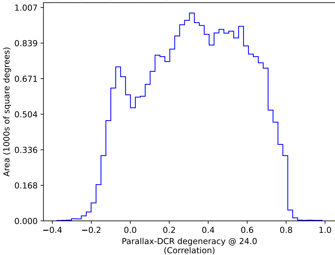
ddf_acor_sf10_ls20_lsr10_v3.4_10yrs : Parallax-DCR degeneracy @ 24.0
