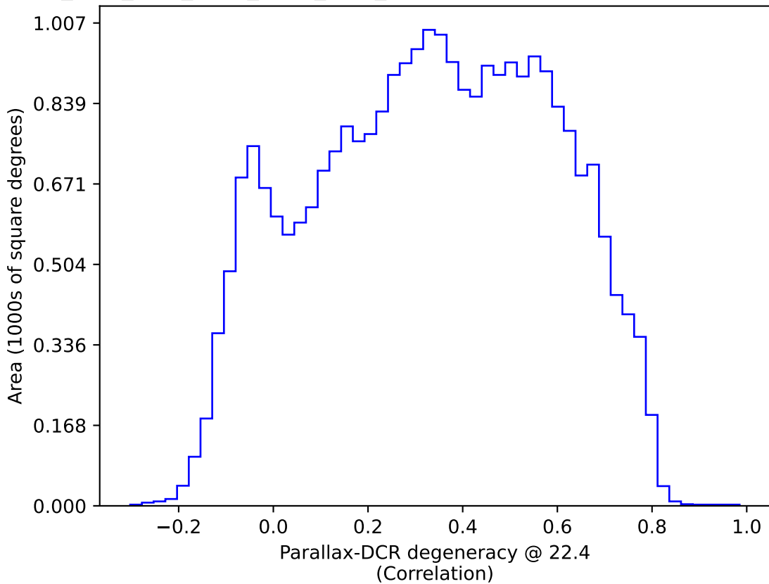
ddf_acor_sf10_lsf20_lsr10_v3.4_10yrs : Parallax-DCR degeneracy @ 22.4
