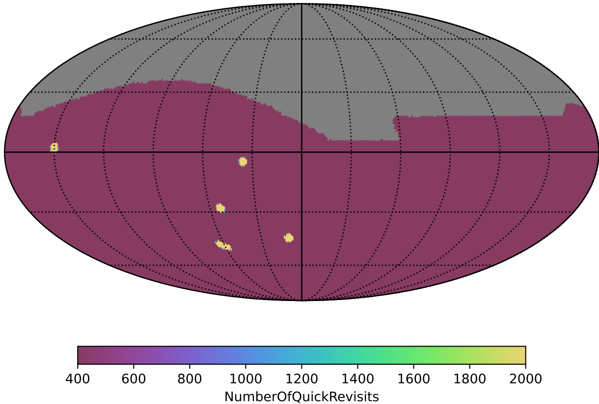
ddf_acor_sf10_lsf20_lsr10_v3.4_10yrs : NumberOfQuickRevisits
